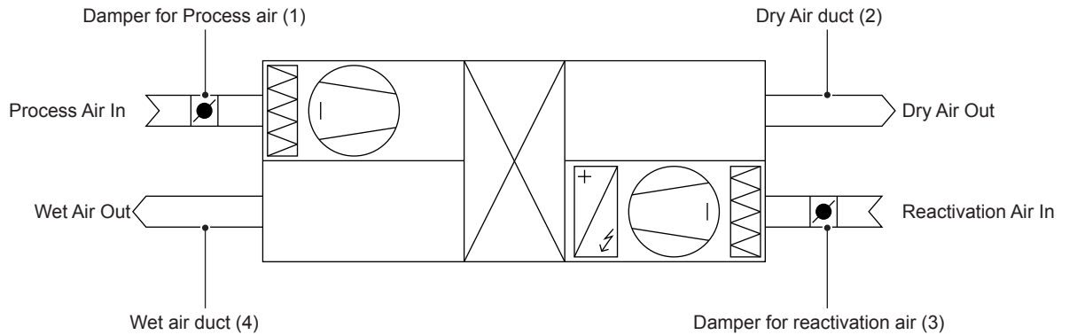
Fig. 3: Installation schematics
